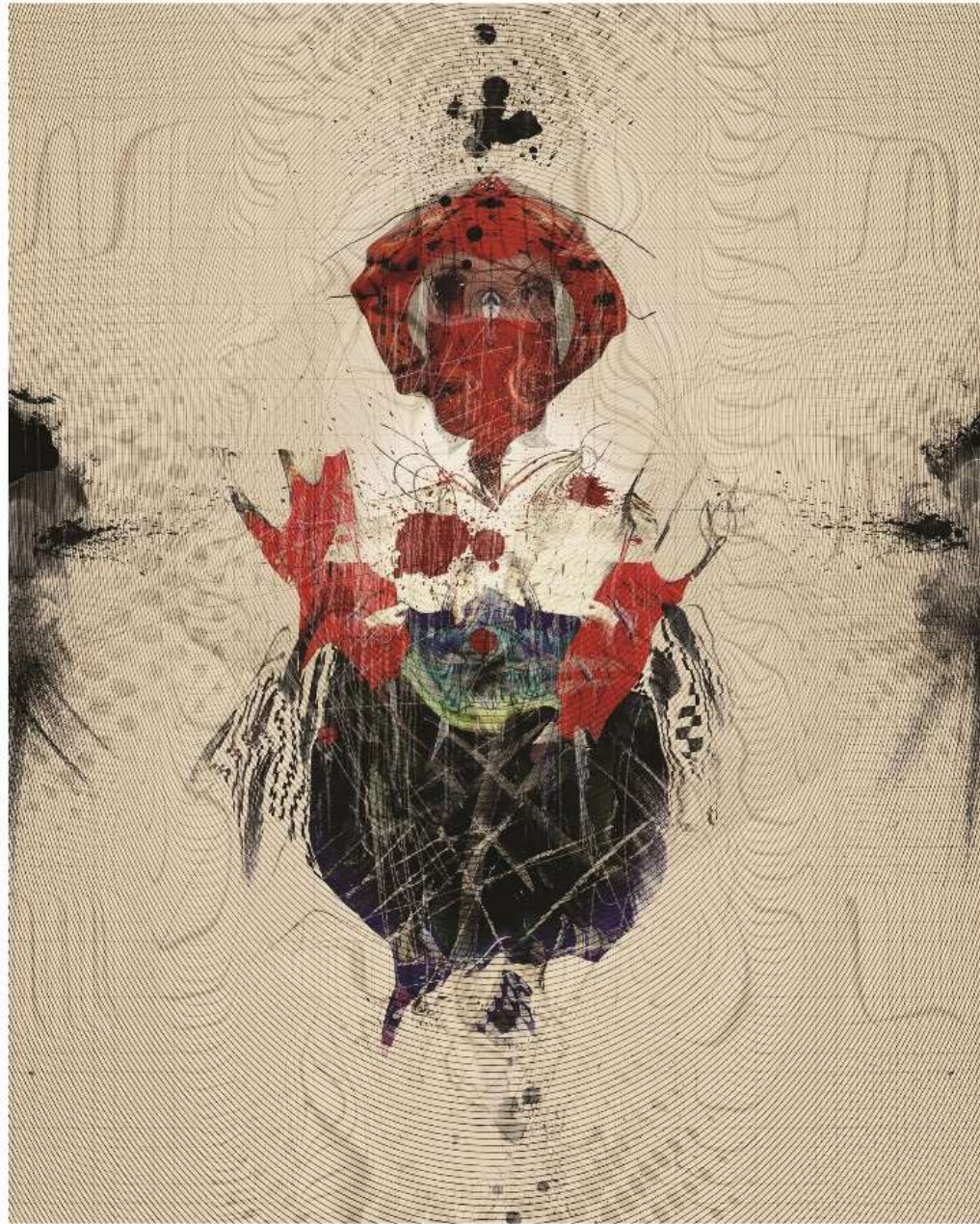
Csaba Pál - Hungary - Open Architecture I
